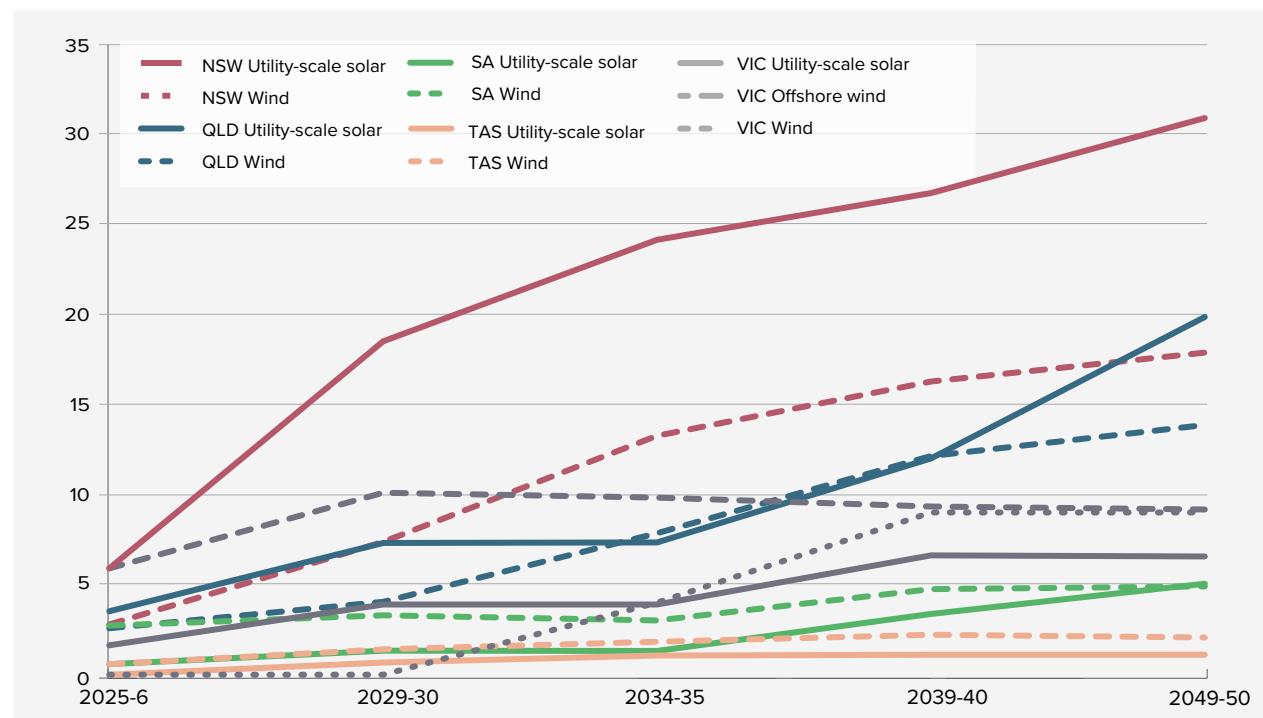
Figure 6: Forecast NEM installed REZ generation capacity (GW) 2026 to 2050, by jurisdiction and technology
