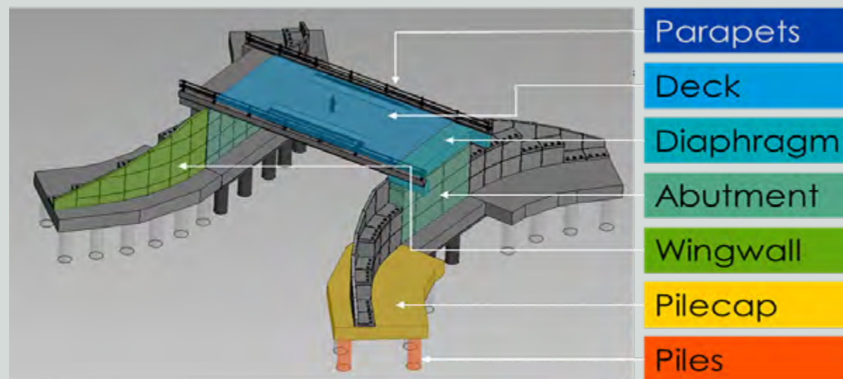
Figure 41: Features of a modular bridge solution
