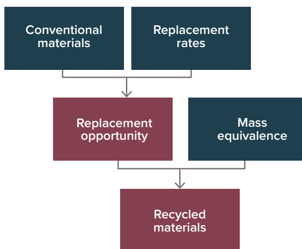
Figure 19: Model map
